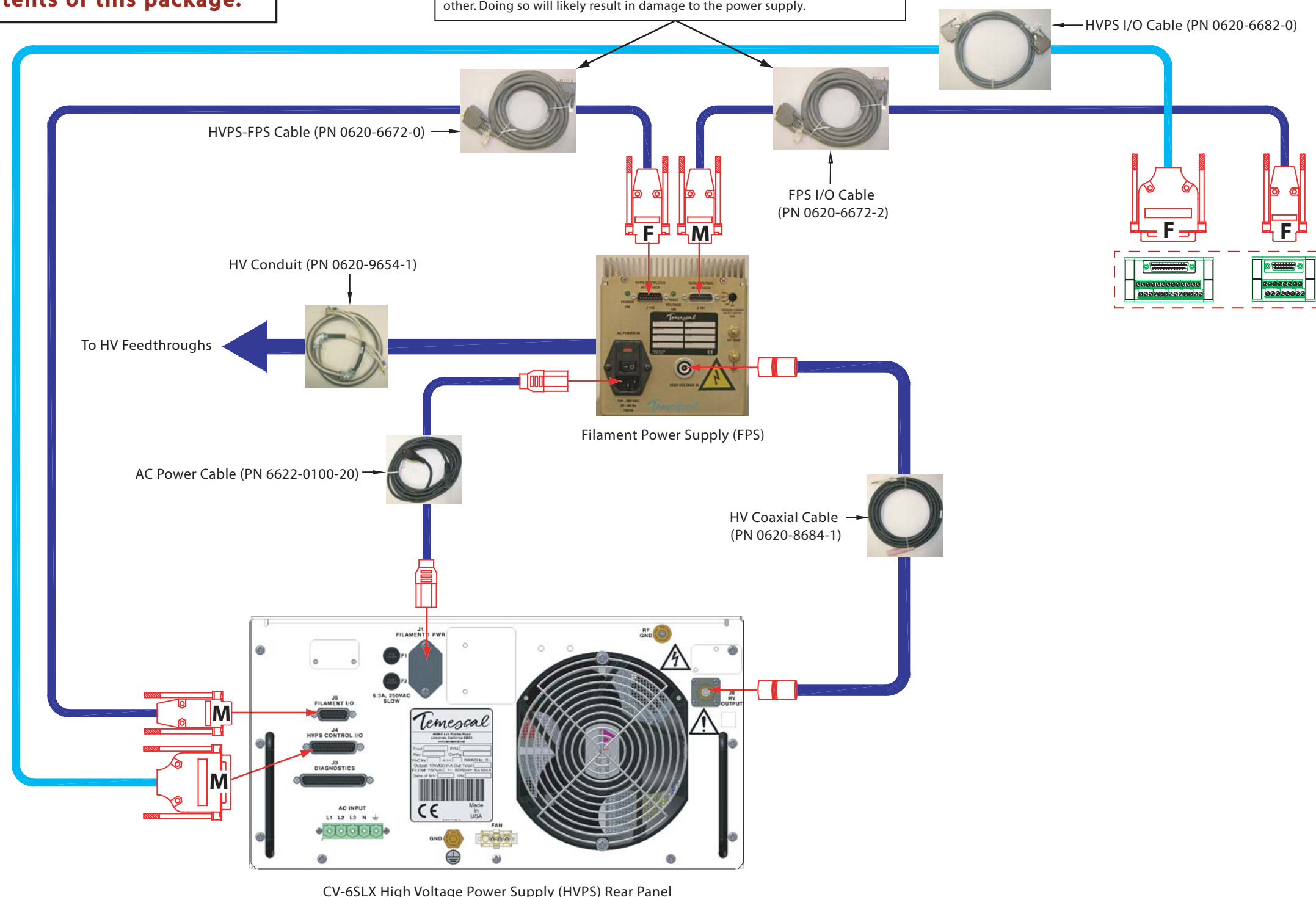
CV-6SLX High Voltage Power Supply (HVPS) Rear Panel
